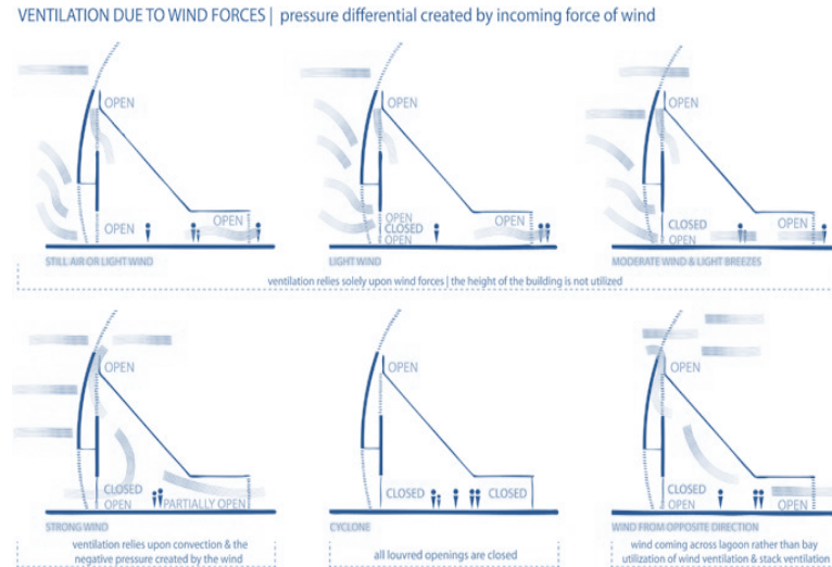
Figure 7: Cultural Center TJIBAOU by RENZO PIANO.
